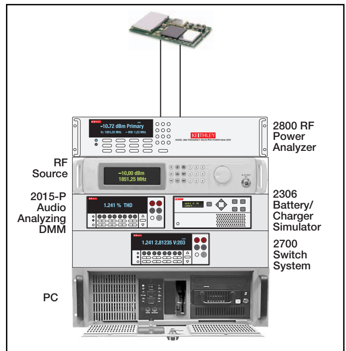
Figure 5. Mobile phone transmitter/receiver board calibration system. A high speed, simplified, low cost solution.
