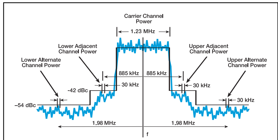
Figure 2. Power spectral density plot of a cdmaOne transmission, showing limits on adjacent channel power and alternate channel power. The Model 2800 can measure all five power levels in a single acquisition.
